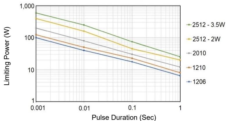
Surge Curve
