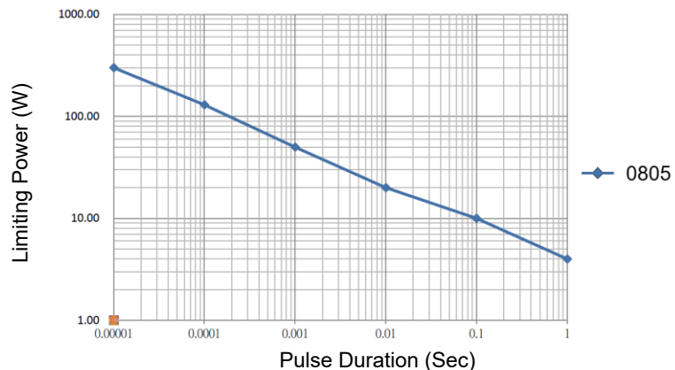
Surge Curve
