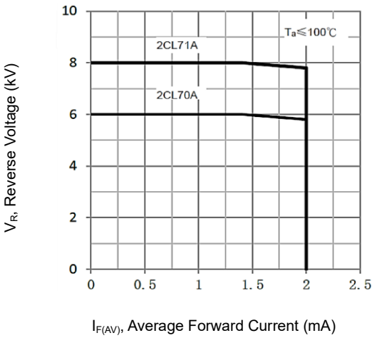
Reverse Voltage vs. Average Forward Current
