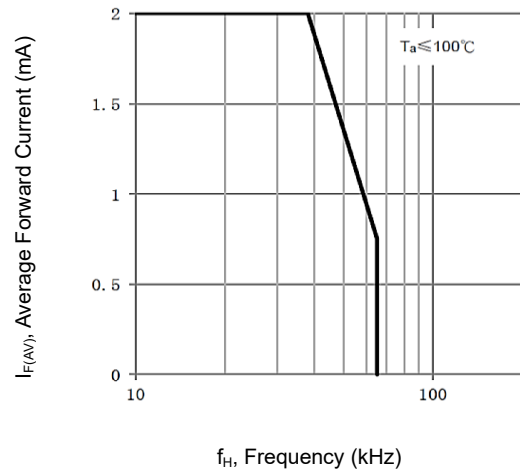
Average Forward Current vs. Frequency
