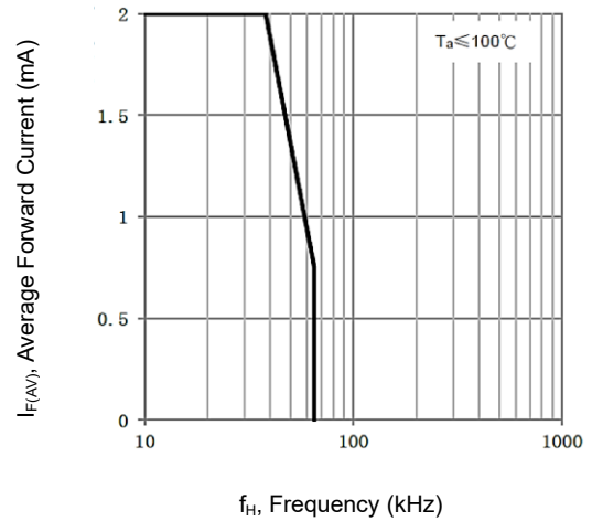
Average Forward Current vs. Frequency
