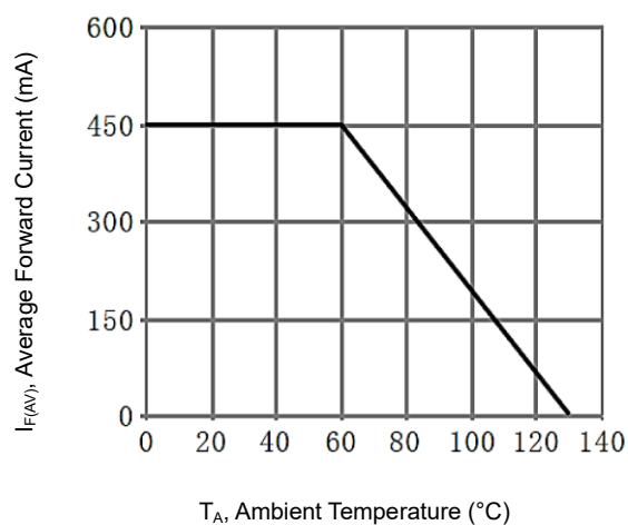
Typical Forward Current Derating Curve
