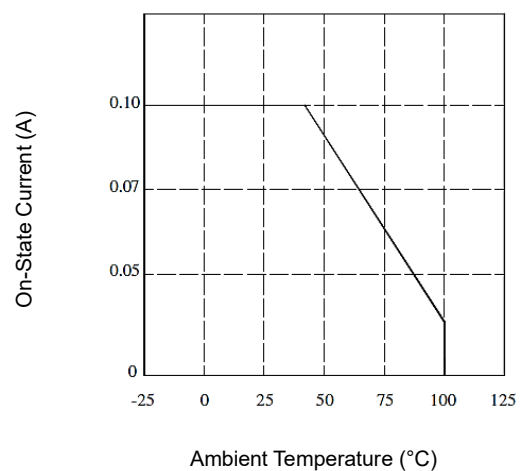
On-State Current vs. Ambient Temperature
