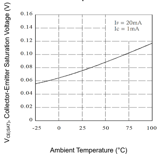
Collector-Emitter Saturation Voltage vs. Temperature
