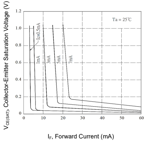
Collector-Emitter Saturation Voltage vs. Forward Current
