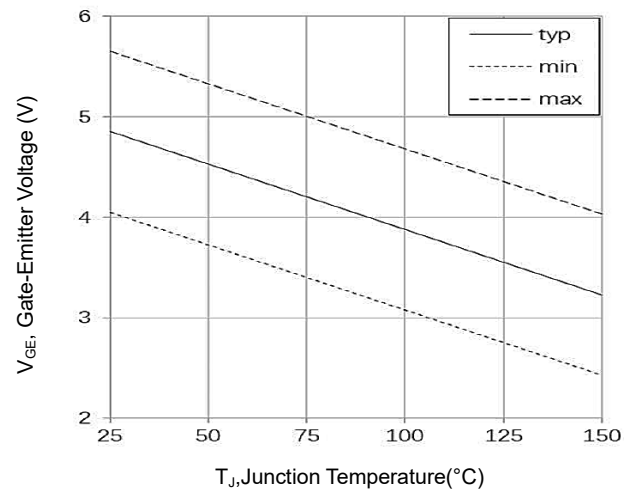
Gate-Emitter Voltage vs Junction Temperature
