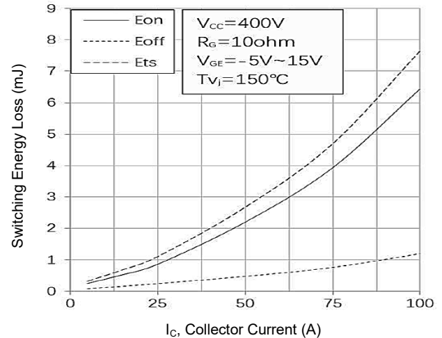
Switching Energy Loss vs Collect Current
