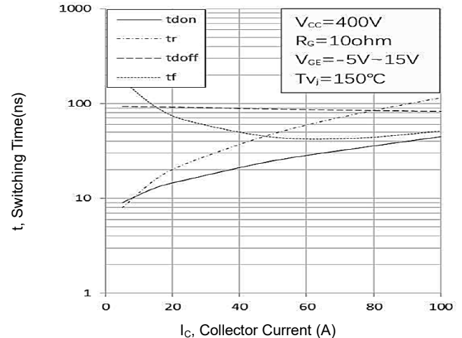
Switching Times vs Collect Current
