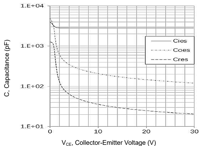
Typical Capacitance
