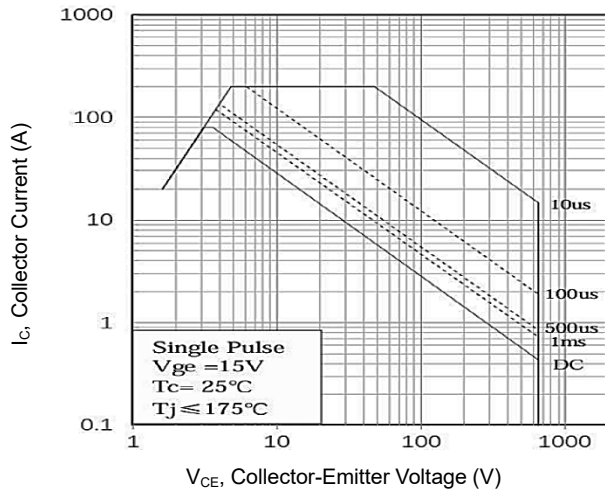
FBSOA
