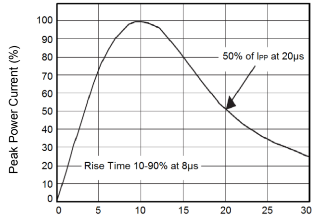
Pulse Waveforms
