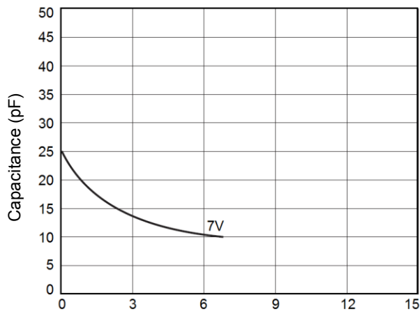
Capacitance vs. Bias Voltage at 1MHz
