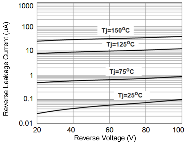
Reverse Characteristics
