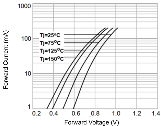
Forward Characteristics
