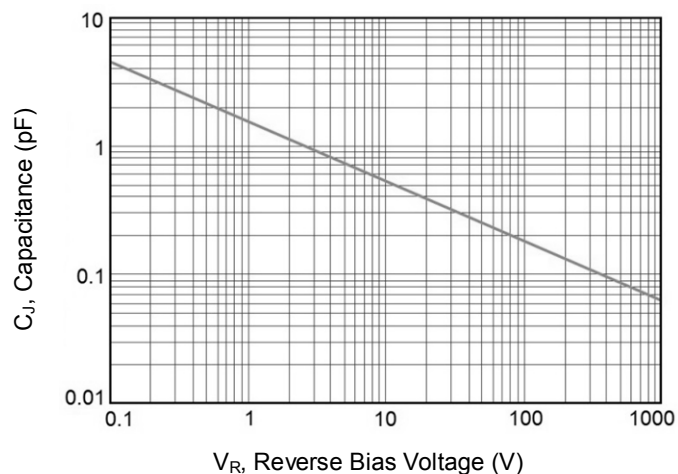
Typical Junction Capacitance Under Bias
