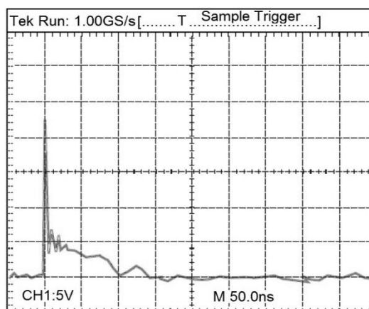
ESD Clamping (8kV Contact IEC61000-4-2)
