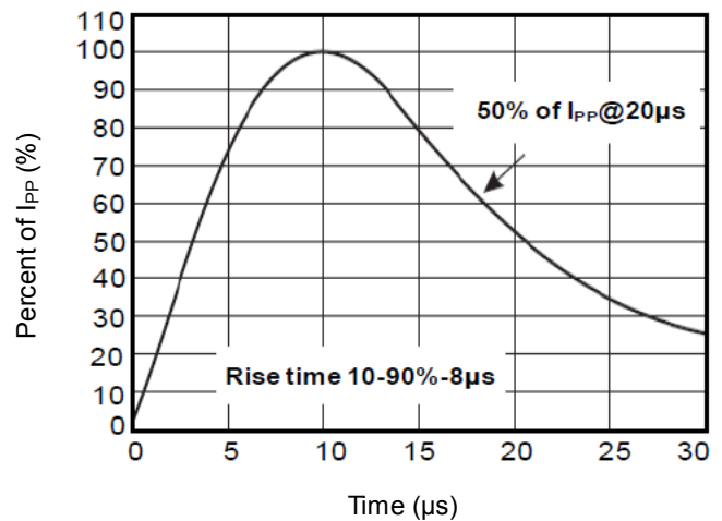
Pulse Waveform
