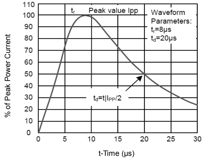
Pulse Waveforms
