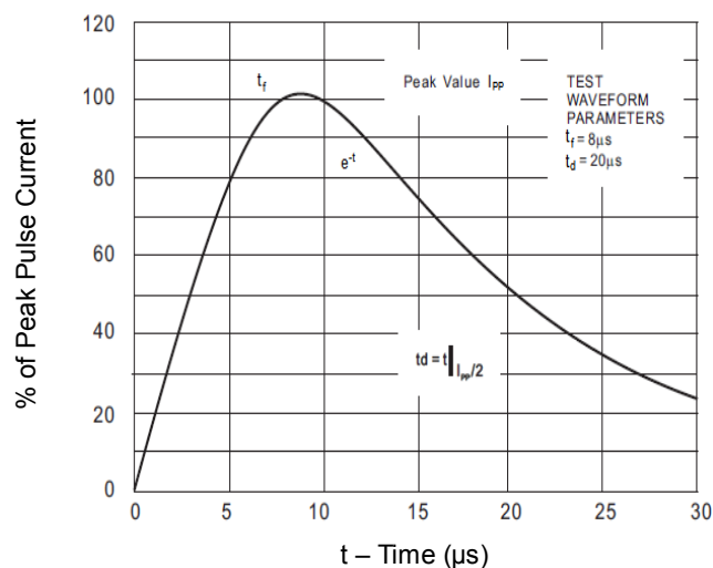
Pulse Waveform
