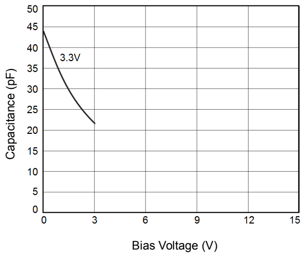
Capacitance vs. Bias Voltage at 1MHz
