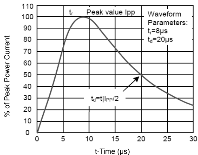
Pulse Waveforms
