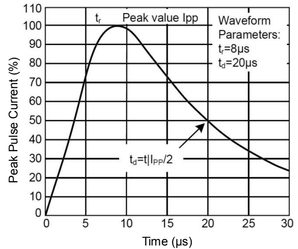
Pulse Waveforms
