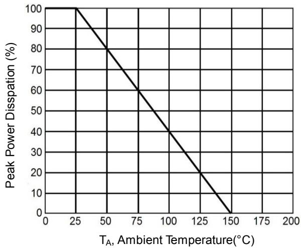
Derating Curve
