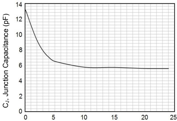
Typical Junction Capacitance(24V)
