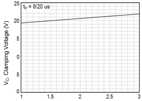
Typical Peak Clamping Voltage(8/2μs)(15V)
