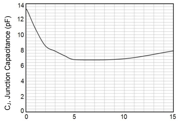
Typical Junction Capacitance(15V)
