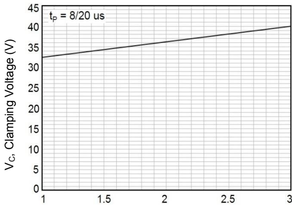
Typical Peak Clamping Voltage(8/2μs)(24V)
