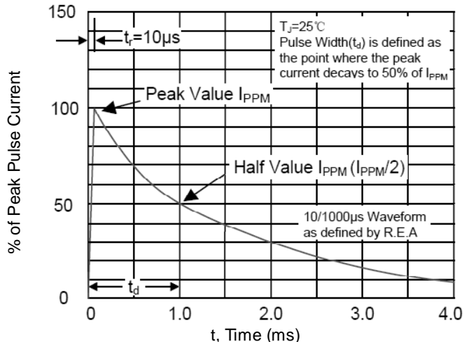
10/1000µs Pulse Waveform
