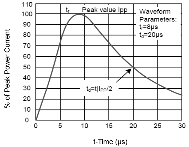
Pulse Waveforms
