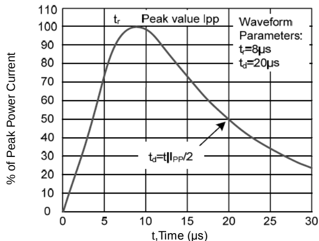
8/20 \mu\text{s} Pulse Waveforms
