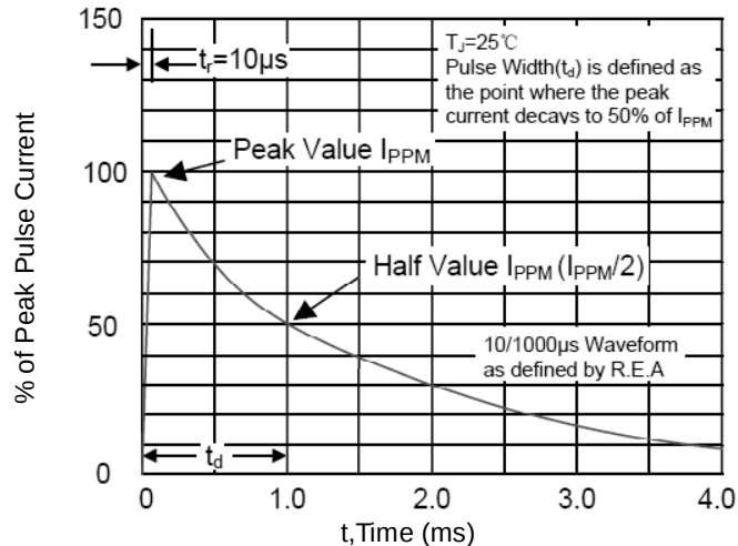
10/1000 \mu\text{s} Pulse Waveform
