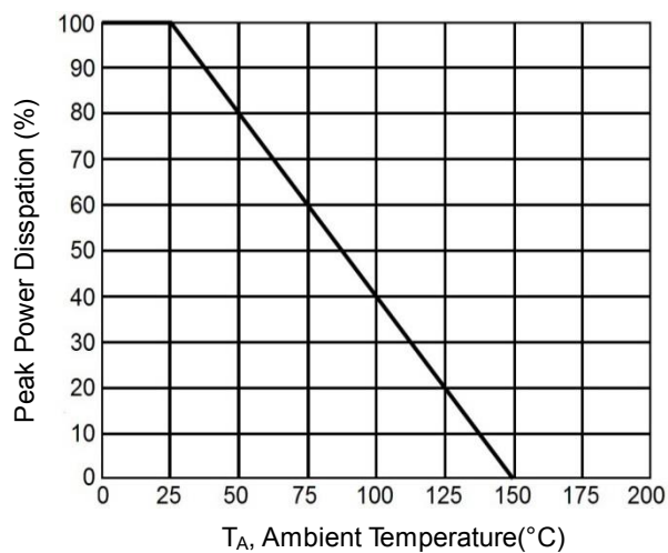
Derating Curve
