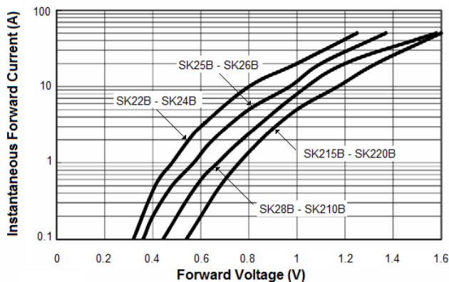
Typical Foward Characteristics
