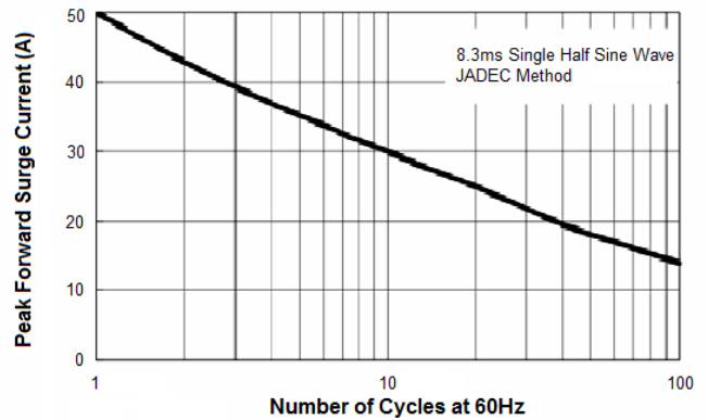
Max Non-Repetitive Forward Surge Current
