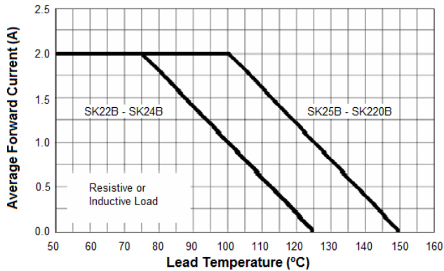
Max Forward Current Derating Curve
